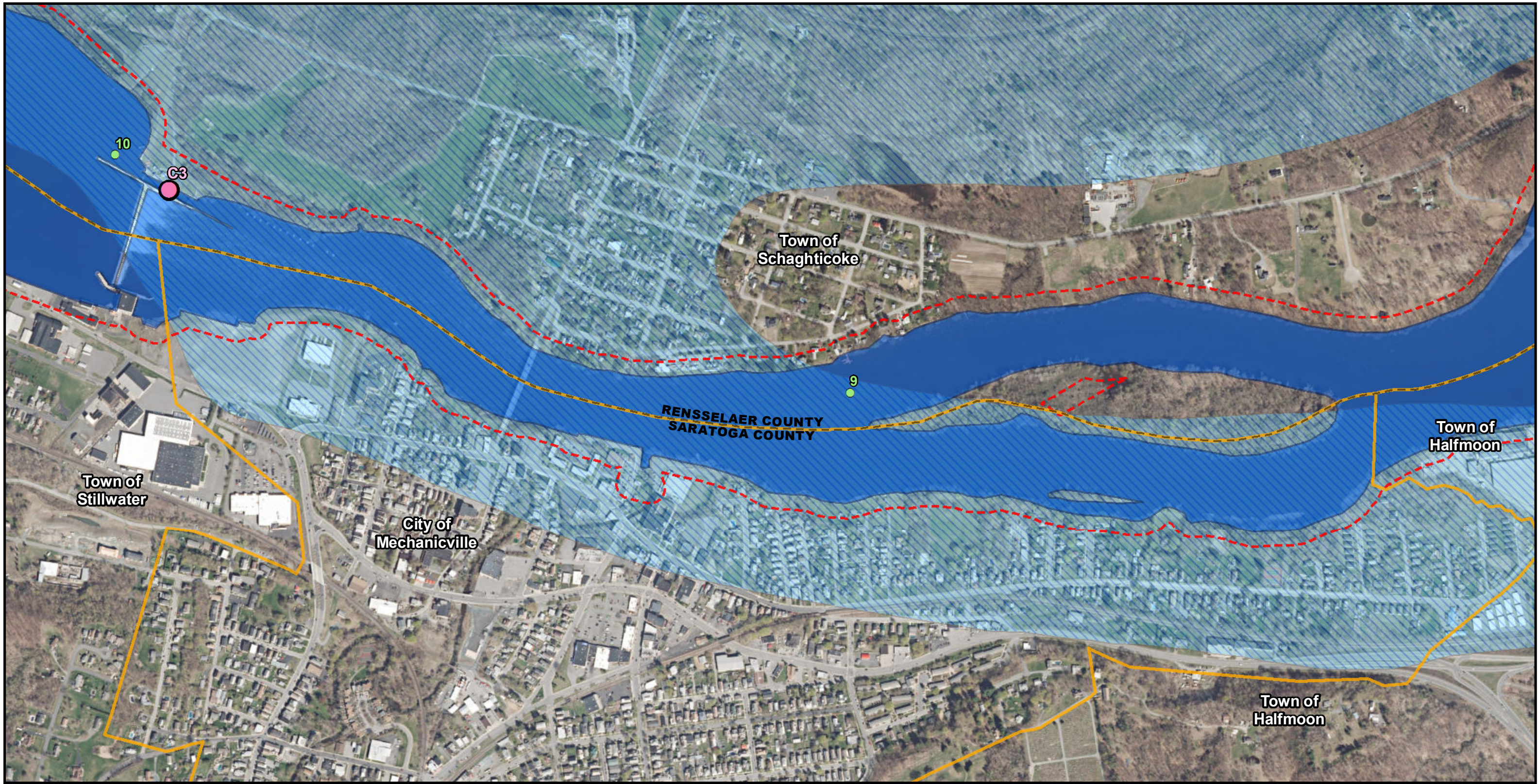
Figure 15F: Aquifers
